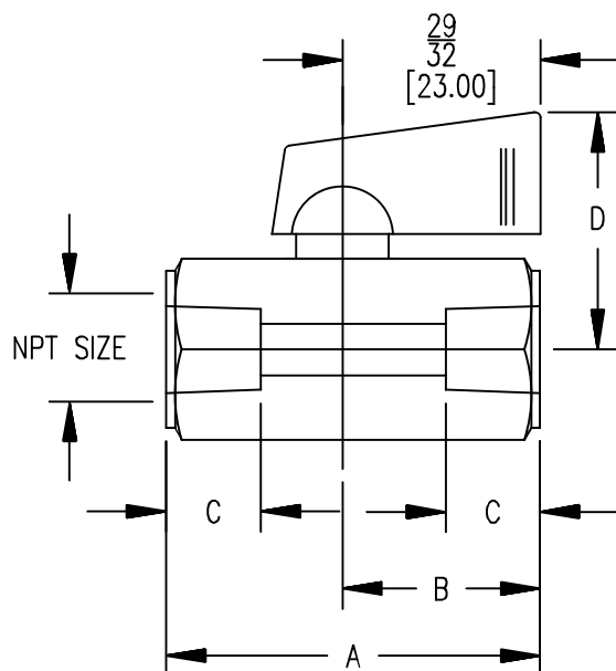
FEMALE X FEMALE CONNECTION SMV2-WFX
