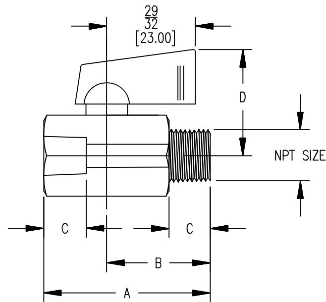
MALE X FEMALE CONNECTION SMV2-WMX
