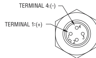
Figure B: Male-12 connector
