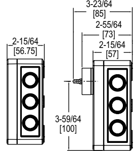
Duct mount
