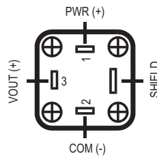
Figure 6a (0-10 VDC)
