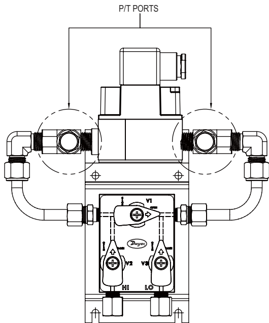
Figure 2: 629HLP-3V P/T ports
