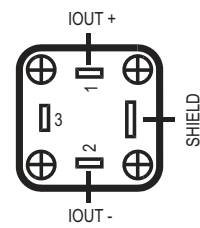
Figure 6b (4-20 mA)
