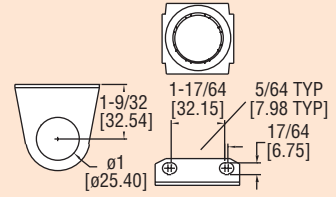
Mounting Bracket For Series 1
