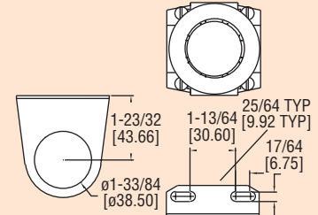
Mounting Bracket For Series 2
